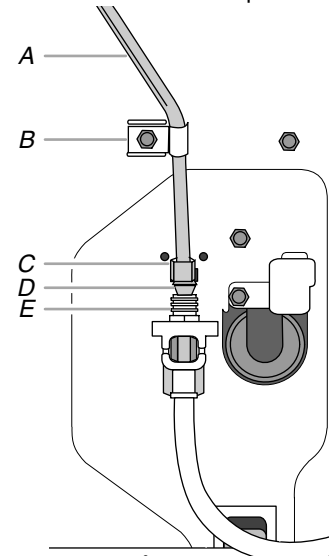
A. Copper tubing B. “P” clamp C. Compression nut D. Compression sleeve E. Water valve inlet port
